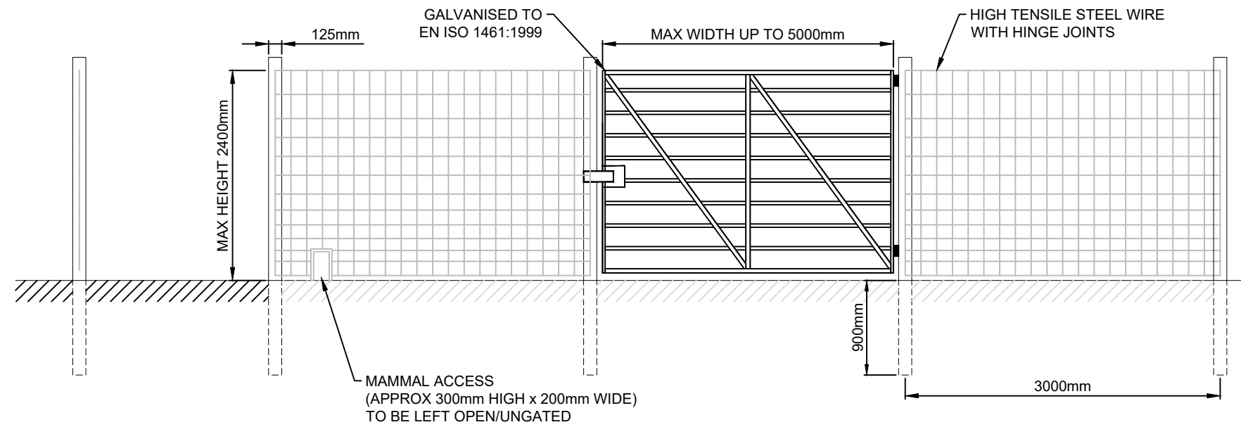
DEER FENCE END ELEVATION
